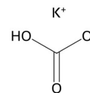
STRUCTURAL FORMULA
