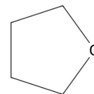
STRUCTURAL FORMULA
